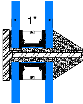
WET GLAZE TO EXT.
