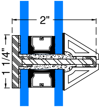
BEVEL METAL STOP TO EXT.
