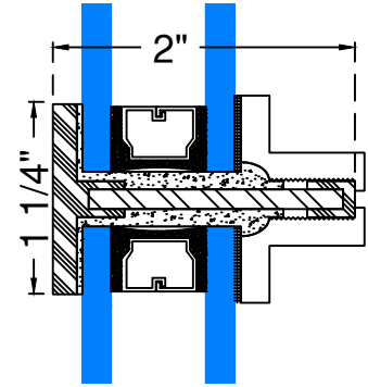
"L" METAL STOP TO EXT.
