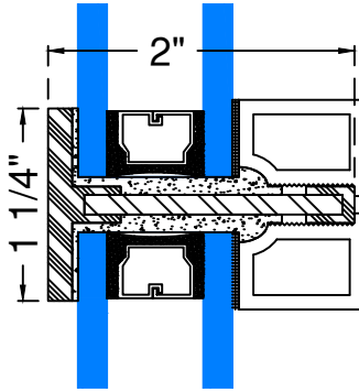
RECTANGLE METAL STOP TO EXT.
