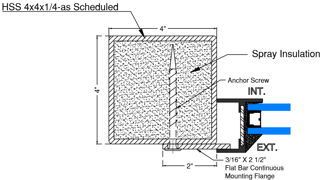
#4 STANDARD FLANGE TO POST
