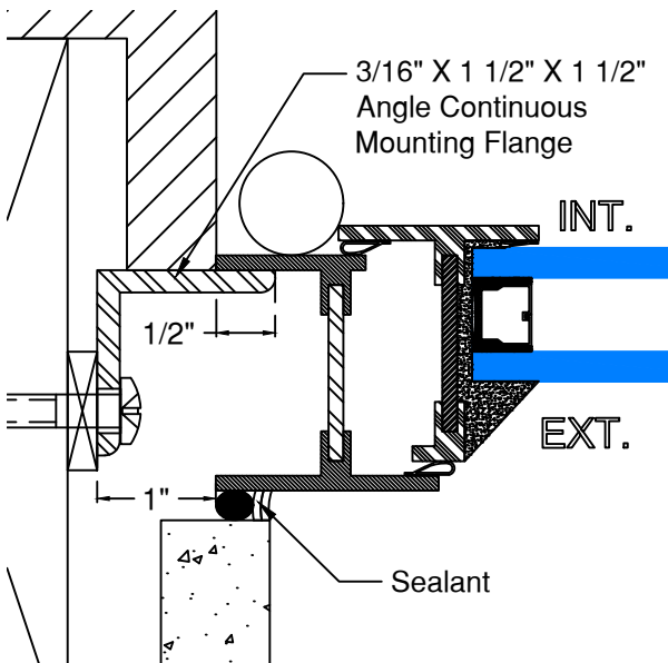
#3 MASONRY FLUSH
