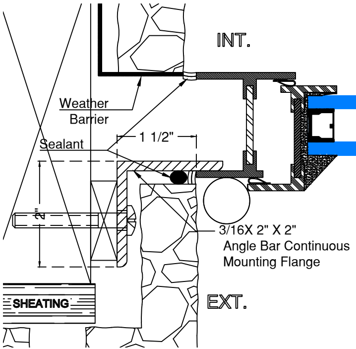
# 7 STONE - LAP
