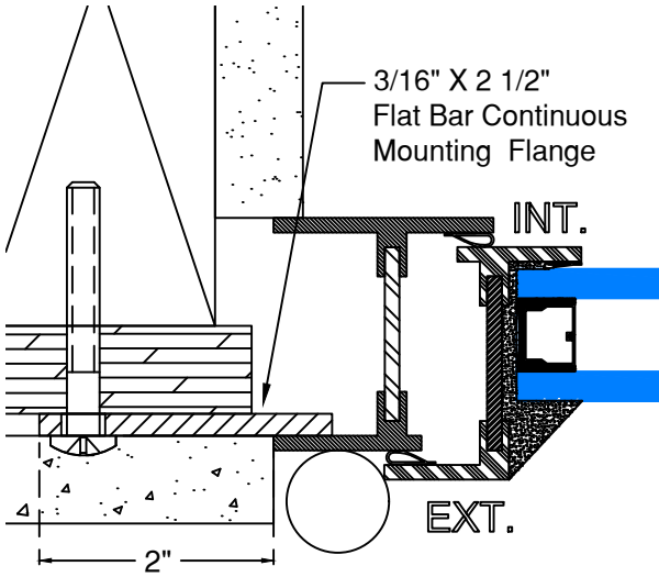
#5 STUCCO / DRYWALL LAP
