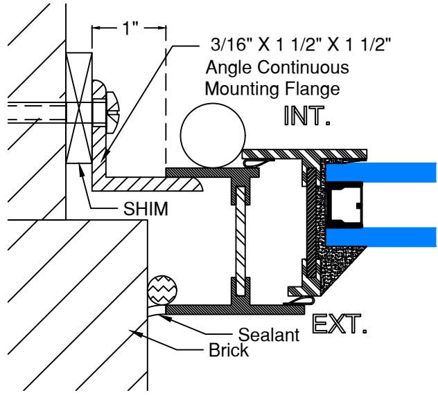
#2 STUCCO / DRYWALL LAP
