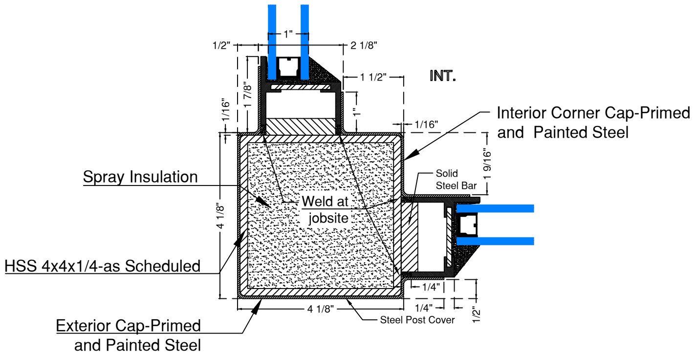
#2 FLANGE WELDED TO COLUMN
