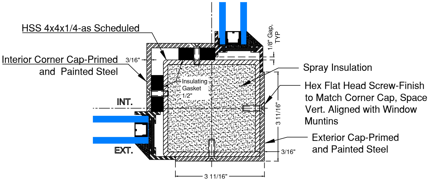
#1 FLANGE WELDED TO COLUMN
