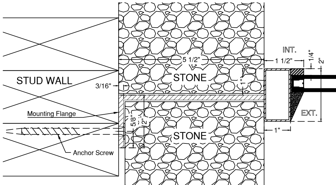
(#4) CUSTOM "L" FLANGE
