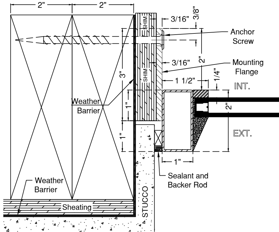
(#4) FLANGE FLUSH TO JAMB
